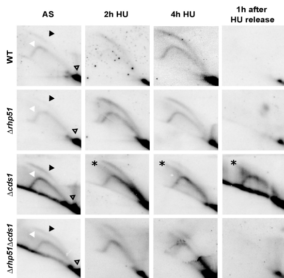
Figure 5. rhp51 deletion partially rescues replication forks in intra-S checkpoint-deficient strain upon HU treatment. 2D gels analysis of replication intermediates at ars2.1 upon HU block and release in wild-type, \Delta cds1 , \Delta rhp51 , and \Delta cds1\Delta rhp51 cells are shown. Note that DNA replication intermediates were enriched by BND-cellulose chromatography, which is responsible for the low signal obtained in G2 cells (30 min after HU release) and the variable levels of 1n DNA (open arrowhead). In wild-type, \Delta rhp51 , and \Delta cds1\Delta rhp51 cells replication intermediates (replication bubbles, black arrowhead; Y-forks, white arrowhead) persist upon HU treatment and disappear after release. In \Delta cds1 cells the bubble arc progressively disappears, and is replaced by double-Ys arcs and X-shaped forms (asterisk) that persist after HU release.
